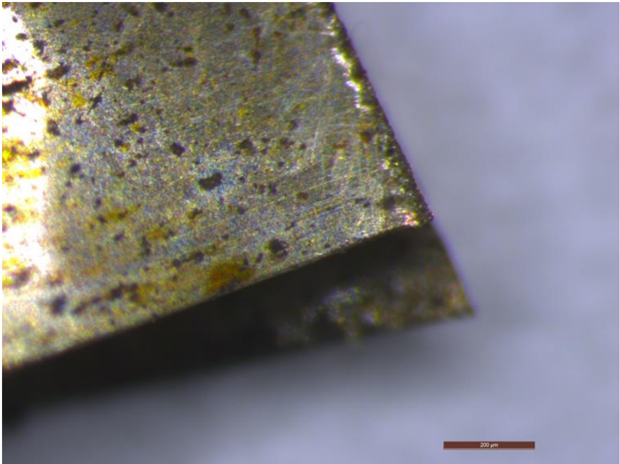
Optical microscopy. Detail-metallic thread
